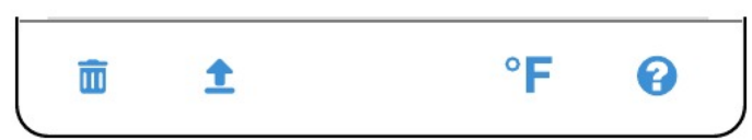
Figure 7 – Android OS
